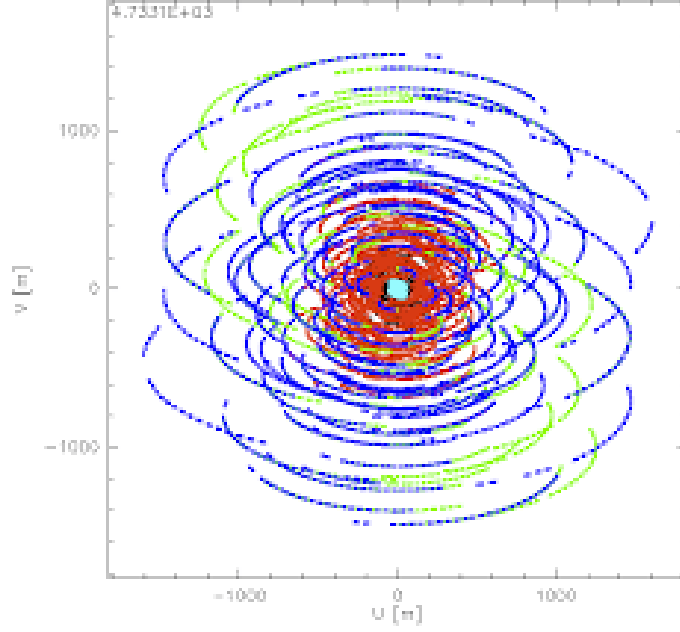
Figure 8: Example UV coverage for an interferometric array over a 6-hour observation.
